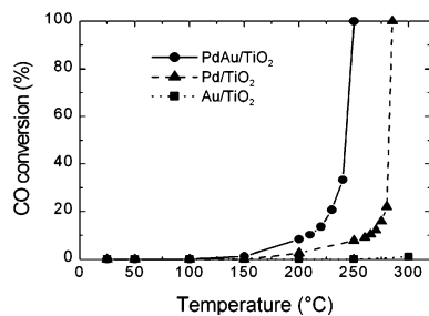
Figure 2. Percentage CO oxidation as a function of temperature for PdAu, Pd-only, and Au-only catalysts supported on TiO 2 . The catalysts were prepared using G4-NH 2 (Pd 27.5 Au 27.5 ), G4-NH 2 (Pd 55 ), and G4-NH 2 (Au 55 ) DENs, respectively. Catalytic reactions were carried out using a 2:1 ratio of O 2 /CO and a gas hourly space velocity of 20 000 cm 3 ·g -1 ·h -1 .
