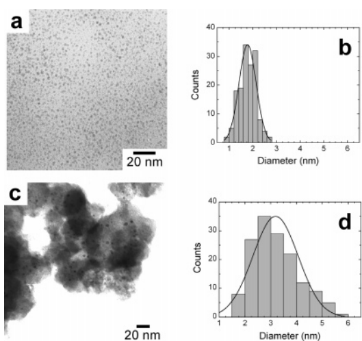
Figure 1. Bright-field TEM images and particle-size distributions for G4-NH 2 (Pd 27.5 Au 27.5 ) DENs prepared by co-complexation of the corresponding metal salts followed by reduction. (a), (b) As synthesized. (c), (d) After incorporation into the titania matrix and subsequent calcination at 500 °C under O 2 and H 2 .
